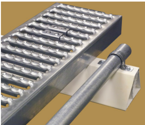
You can even use the Unipier support for multiple tasks. Here we have a grating walk and a piece of electrical conduit attached to the sleeper.
