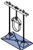
Single Base Trapeze Page 14
