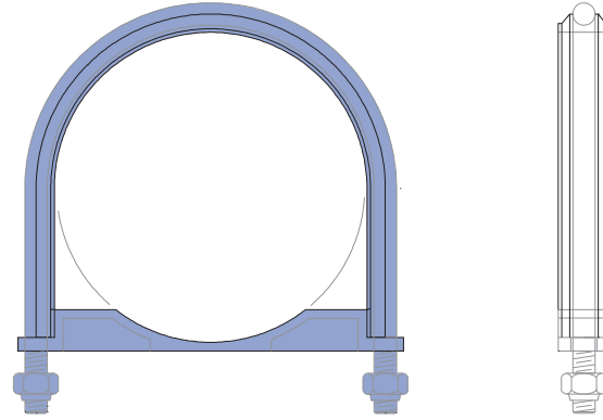
8" thru 12" assembly.
