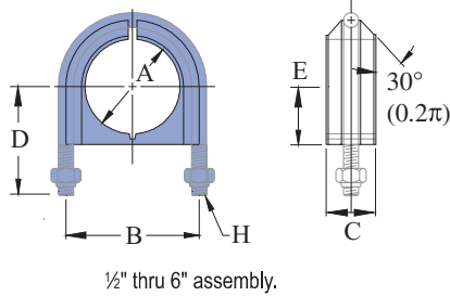
1/2" thru 6" assembly.
