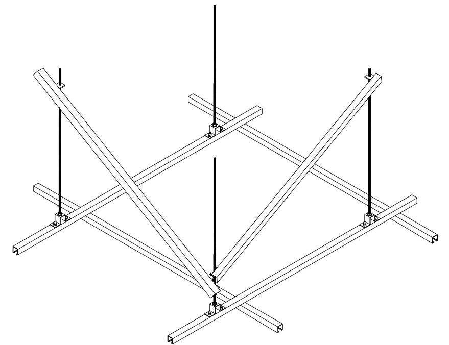
TYPICAL GRID-PARTIAL ISOMETRIC
