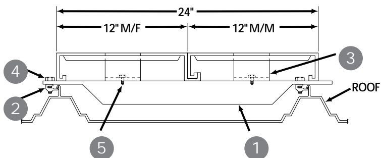
PARALLEL SUPPORT PLATE ASSEMBLY
