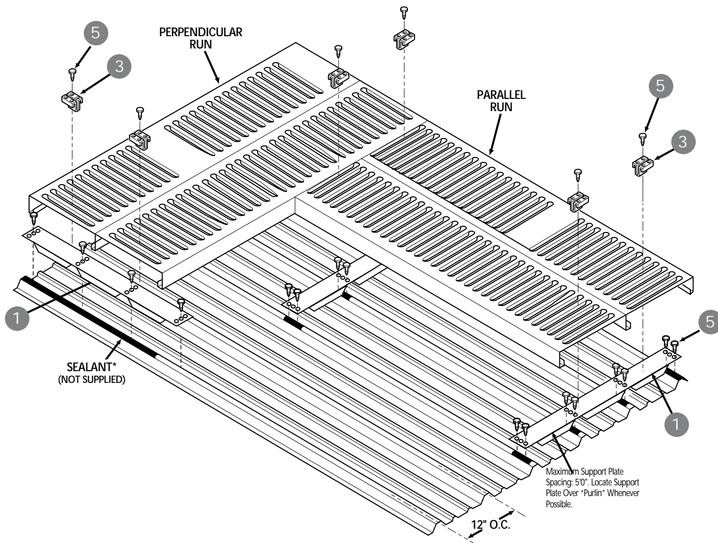
PARALLEL SUPPORT PLATE ASSEMBLY
