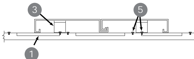
PERPENDICULAR BOLT ASSEMBLY
