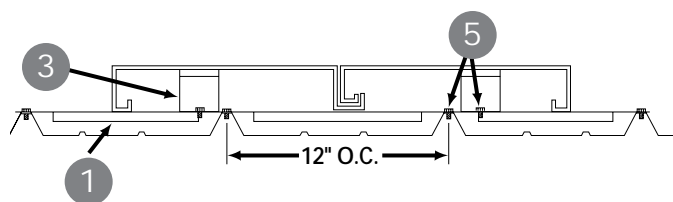
PARALLEL SUPPORT PLATE ASSEMBLY
