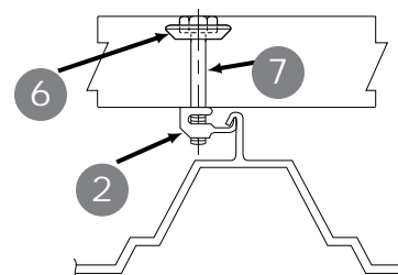
PERPENDICULAR BOLT ASSEMBLY
