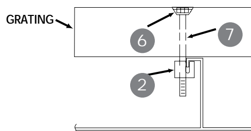
PERPENDICULAR BOLT ASSEMBLY
