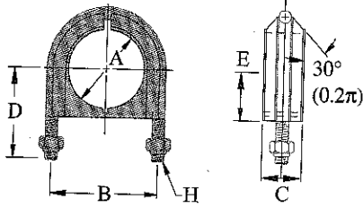
\frac{1}{2} " thru 6" assembly.
