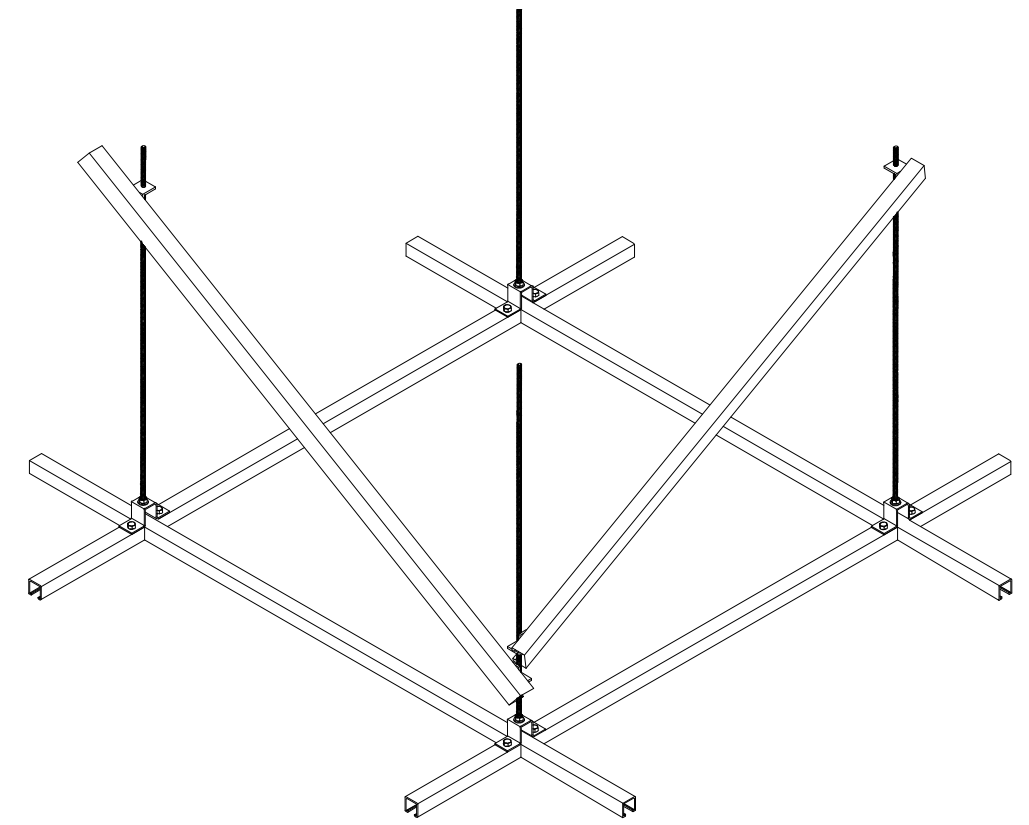
TYPICAL GRID-PARTIAL ISOMETRIC NOT TO SCALE
