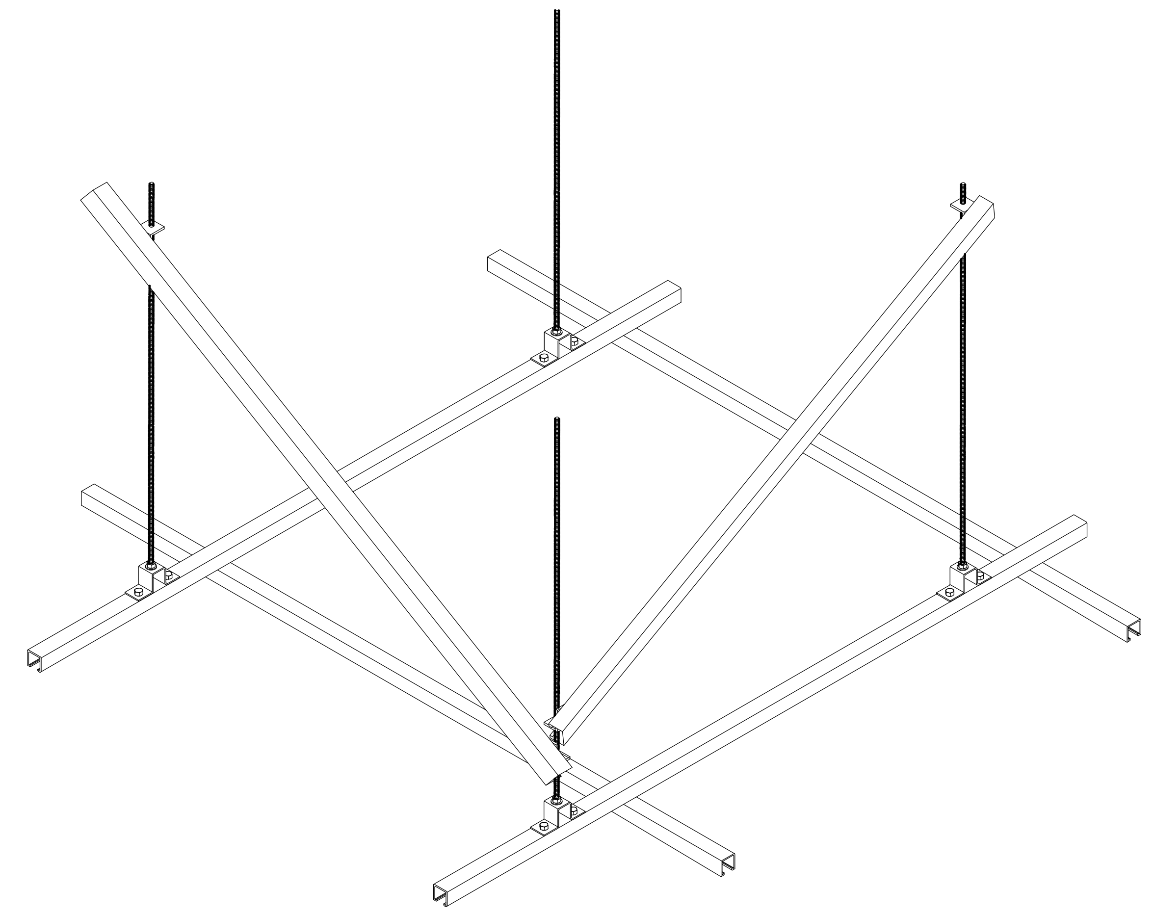
TYPICAL GRID-PARTIAL ISOMETRIC NOT TO SCALE
