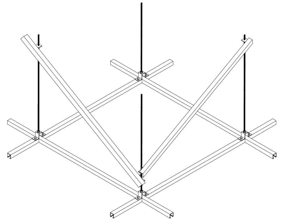
TYPICAL GRID-PARTIAL ISOMETRIC NOT TO SCALE
